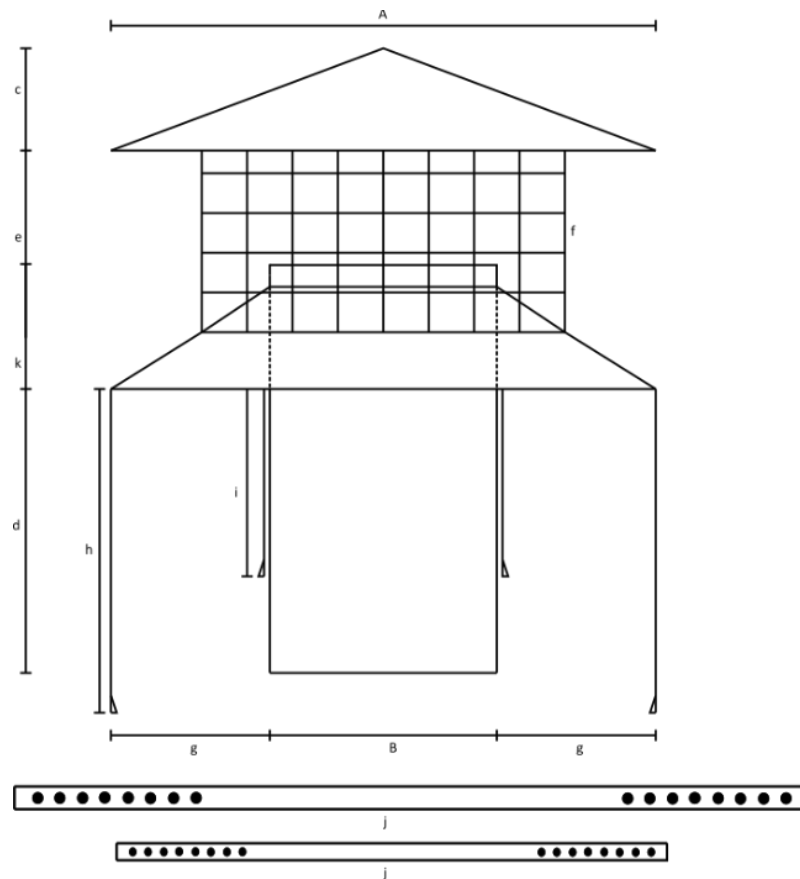
Pot Hanging Cowl - diagram
